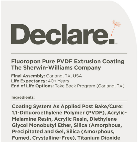
Figure 3: LBC Compliant Sherwin-Williams Coil Coatings Fluoropon Pure PVDF Extrusion Coating system: applied after curing and baking; includes extrusion primer 732X1023FP and all Fluoropon Pure Extrusion topcoats.
