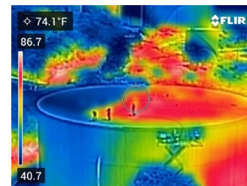
Figure 1 FLIR imaging of this ground storage tank being covered with a TIC demonstrates how well the coated areas (blue and green) retain heat compared to the noncoated areas (red and yellow).
