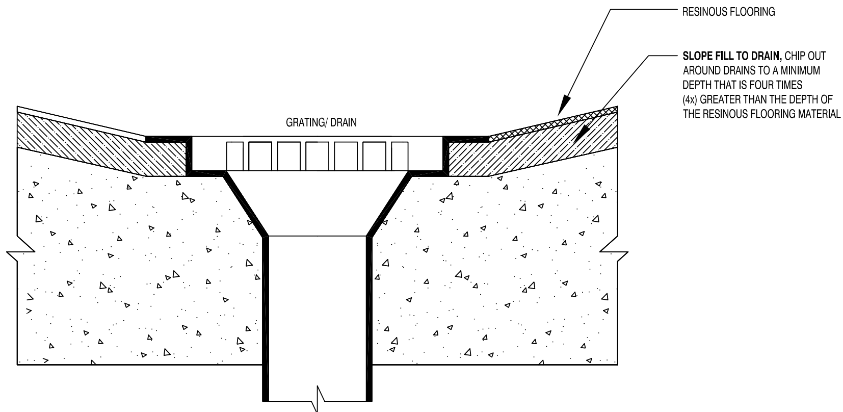
D2 DRAIN DETAIL NTS
