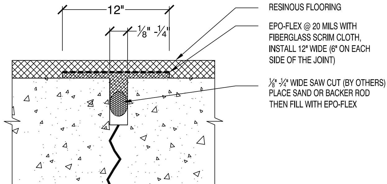
J4 CONCRETE COLD JOINT DETAIL NTS
