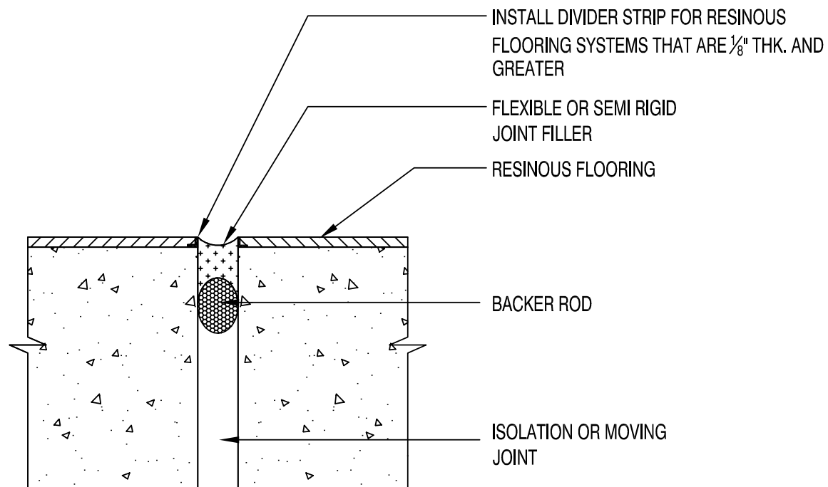
J2 ISOLATION/ MOVING JOINT DETAIL NTS
