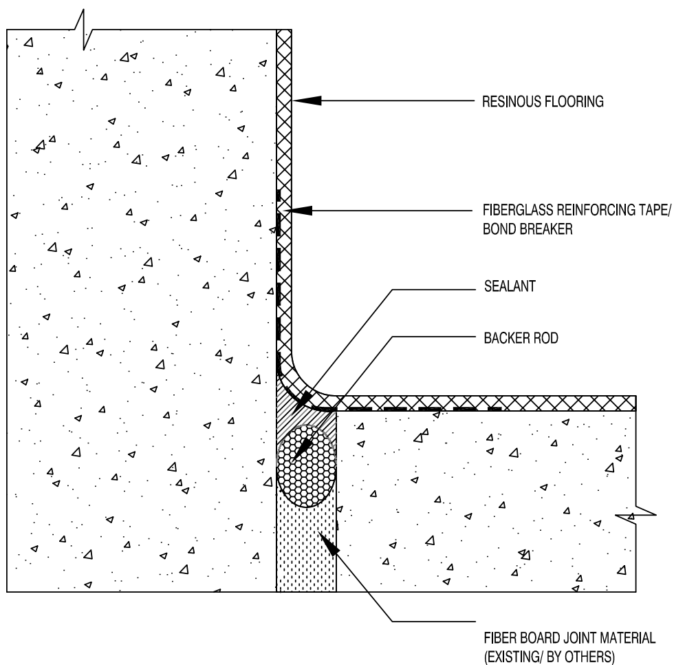
CB3 BRIDGED COVE ISOLATION JOINT 3" = 1'-0"
