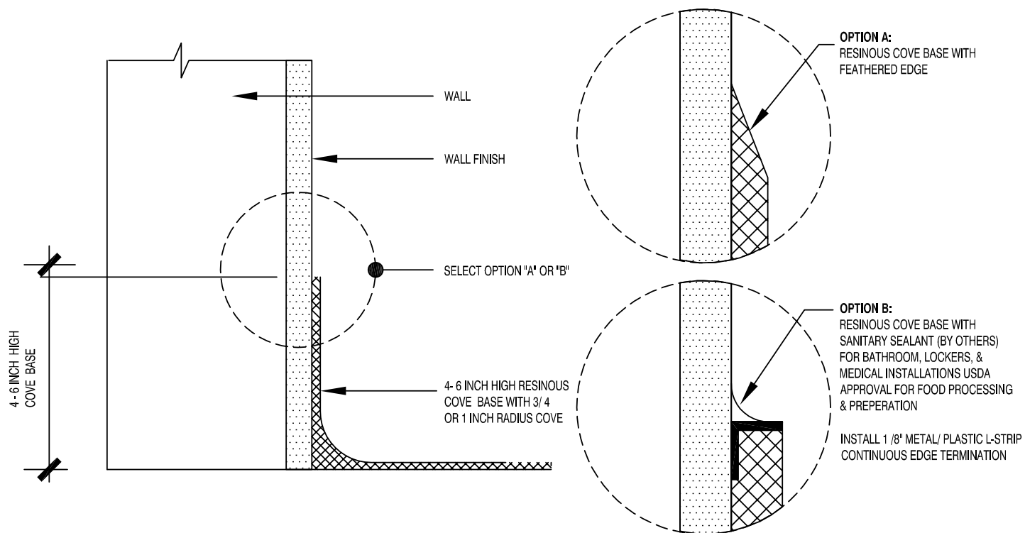
CB5 COVE BASE TERMINATION NTS
