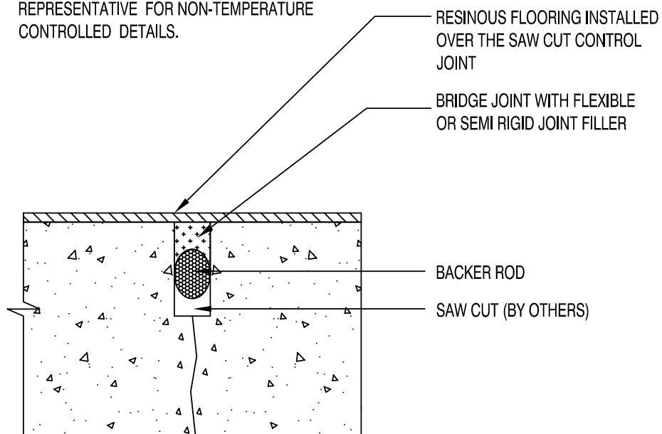
J3 SAW CUT CONTROL JOINT DETAIL NTS
