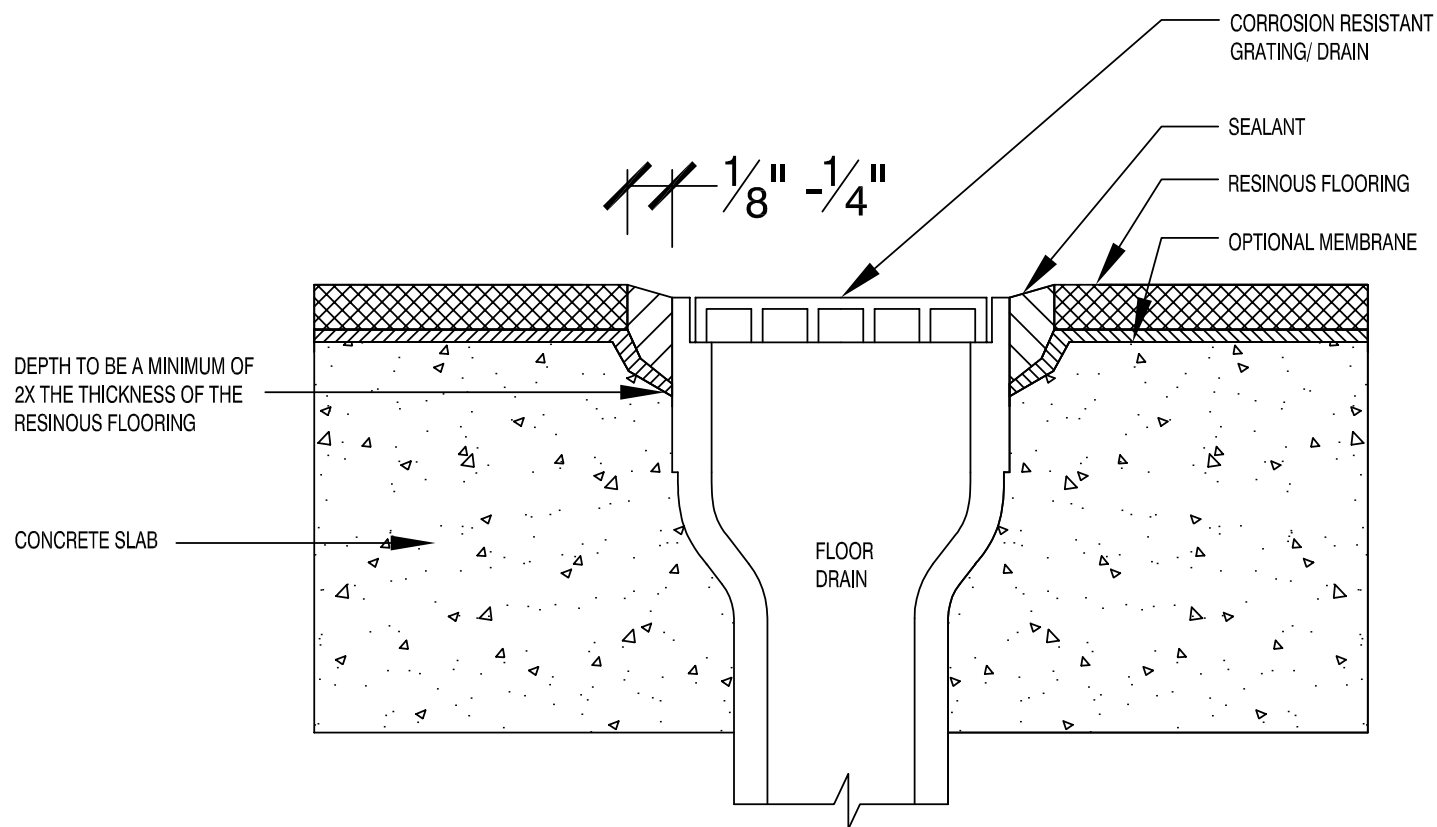
D1 DRAIN DETAIL IN TEMPERATURE ENVIRONMENT NTS
