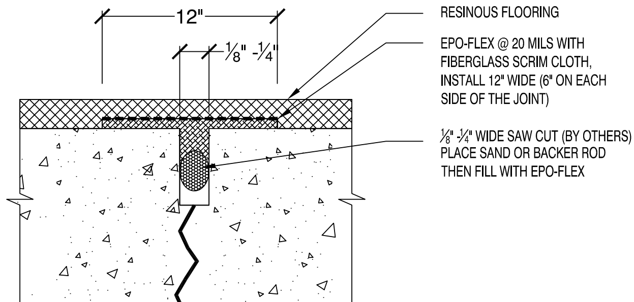
J4 CONCRETE COLD JOINT DETAIL NTS
