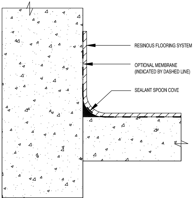
CB4 COVE BUTT JOINT HALF FULL SCALE
