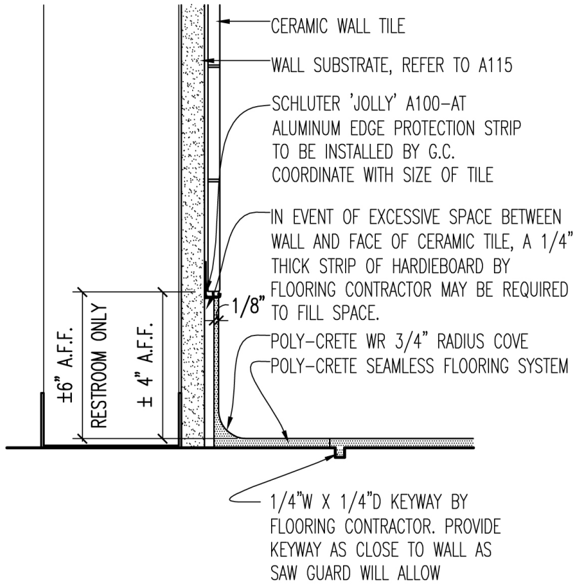
9A A125 POLYCRETE BASE DETAIL @ TILE TO POLYCRETE 3" = 1'-0"
